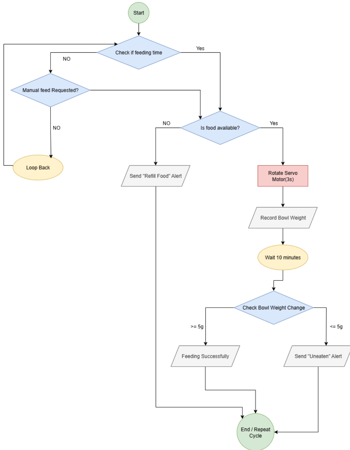
Figure 2: System Flowchart
